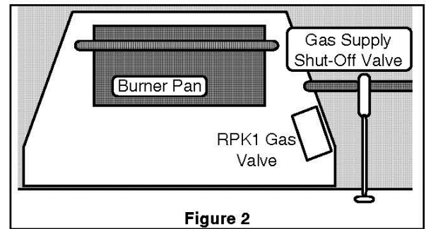
RPK1 Valve Placement Options (as viewed from above) ← Valve Assembly outside firebox. Forward and to the Side of the burner pan. →
