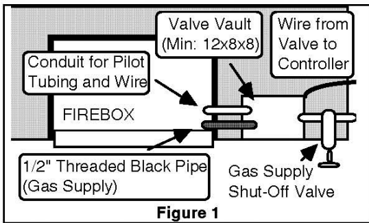
RPK1 Valve Placement Options (as viewed from above) ← Valve Assembly outside firebox. Forward and to the Side of the burner pan. →
